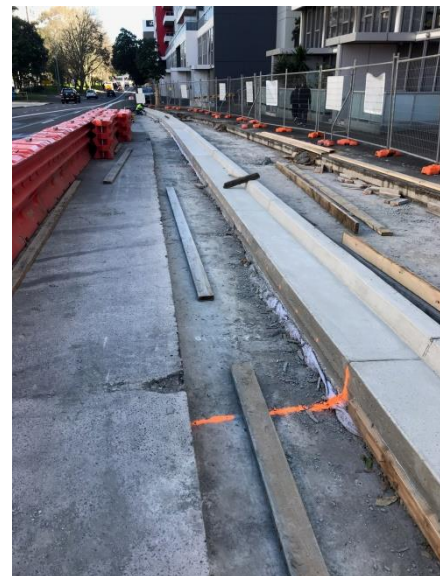
Photo above – Section of completed kerb and gutter and road section on Lachlan Street
